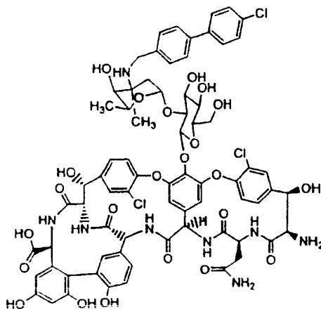
Des-leucyl chlorobiphenyl vancomycin
